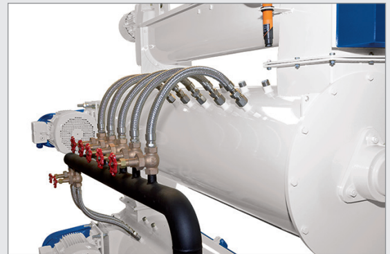
Steam injection system
